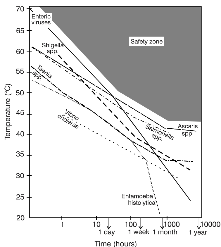
Figure 5.1 Time-temperature requirements for pathogen inactivation (Strauch, 1991; Carrington, 2001)
