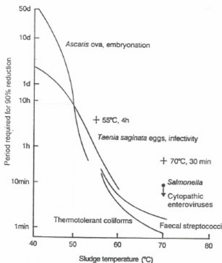
Figure 5.2 Time-temperature requirements for 90% pathogen inactivation. Crosses relate to temperature/time conditions specified in the UK Code of Practice (Bruce et al. , 1990)
