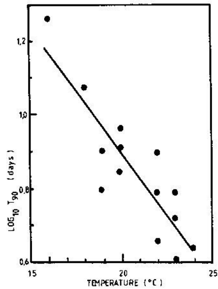
Figure 5.3 Effect of storage temperature on the decimal reduction time, T_{90} , of salmonellas in stored digesting sludge (Pike, 1983)
