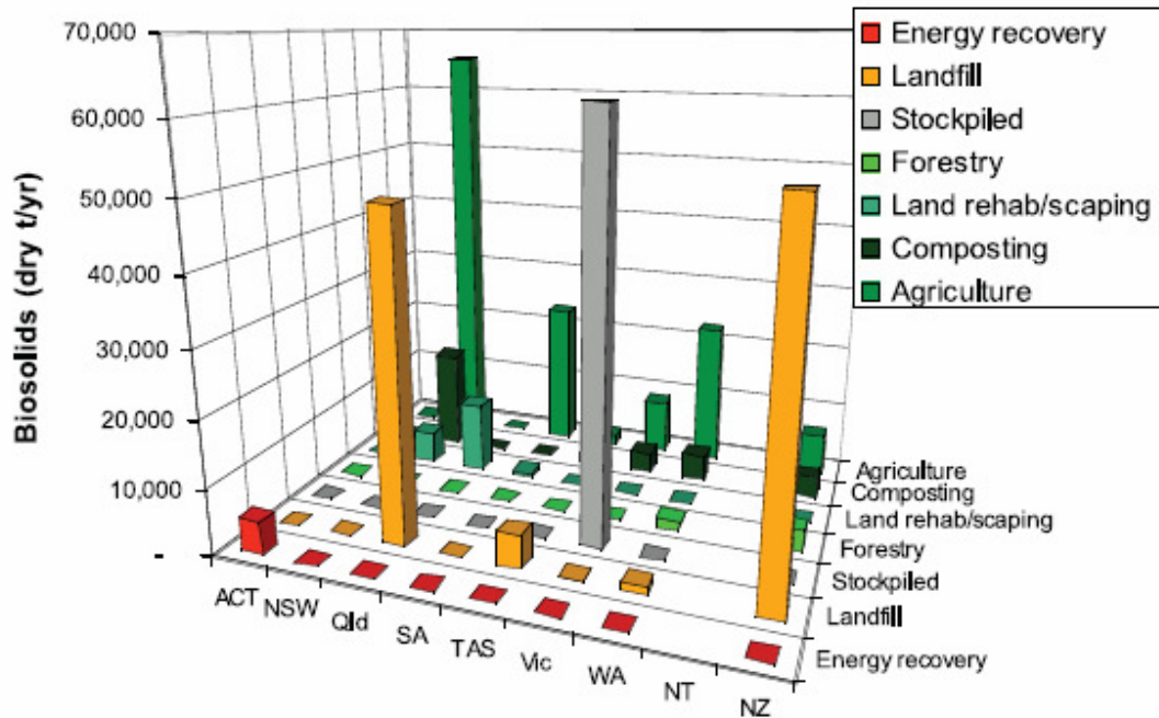
Figure 2.6 Biosolids end uses in Australia and New Zealand (Gale, http://www.bvsde.paho.org/bvsaar/cdlodos/pdf/theaustralasian109.pdf )
