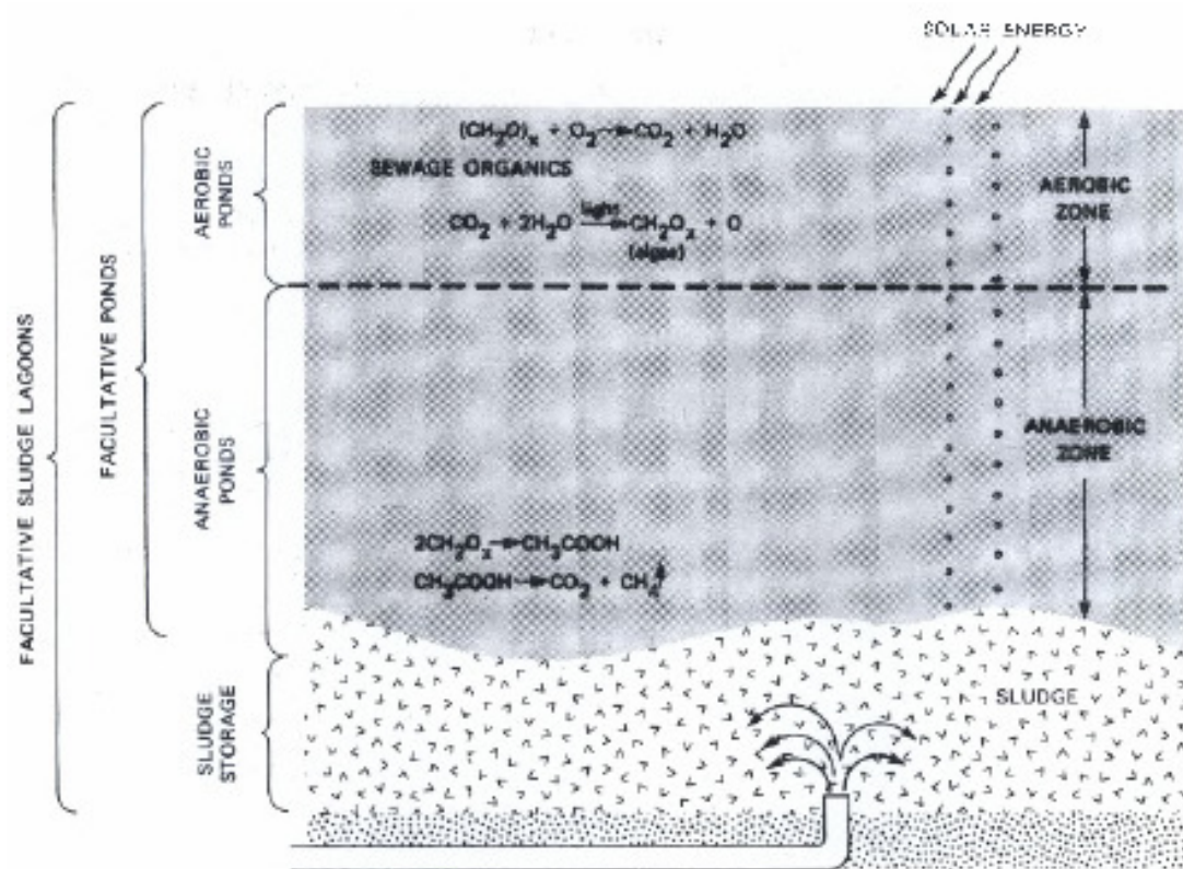
Figure 3.2 Facultative sludge lagoon with aerobic and anaerobic phases (US EPA, 1979)
