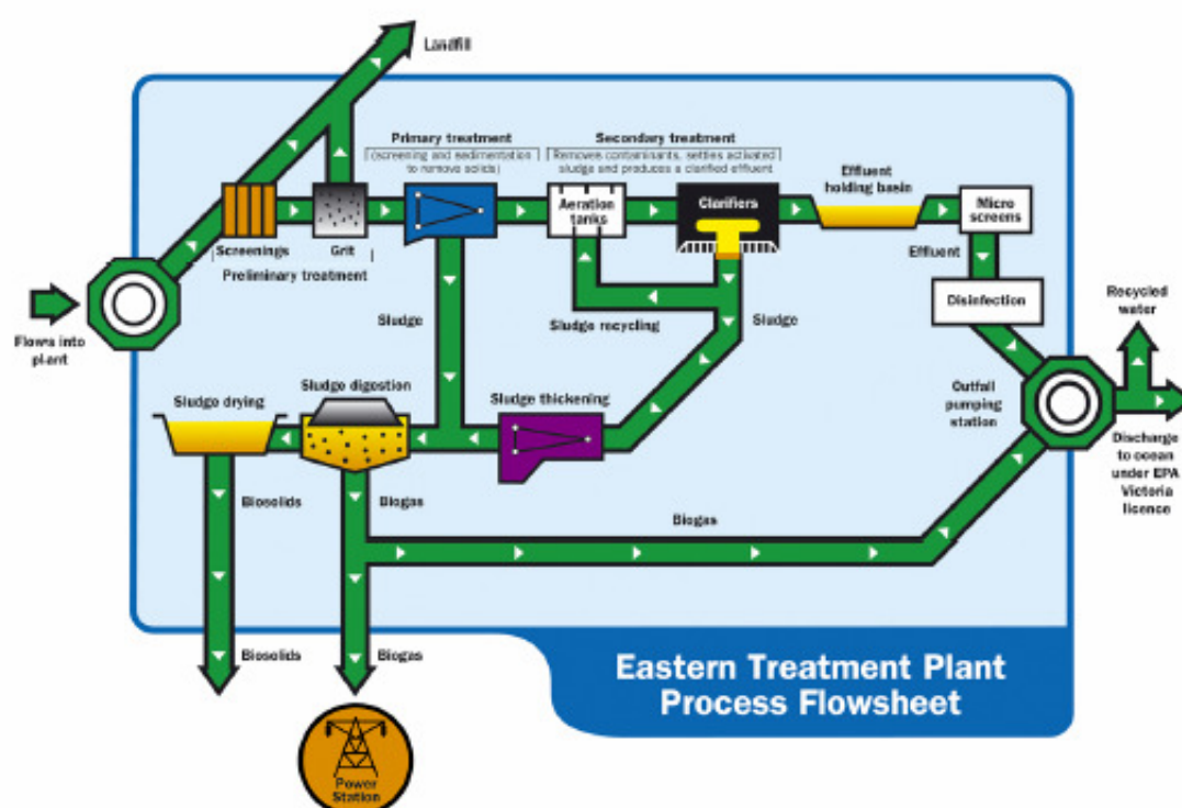
Figure 2.3 Sewage treatment at the Eastern Treatment Plant (Melbourne Water, 2005)
