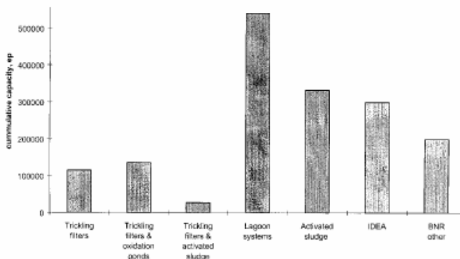
Figure 2.4 Wastewater treatment by different methods operated by other Water Service Providers (Van Oorschot et al. , 2000)
